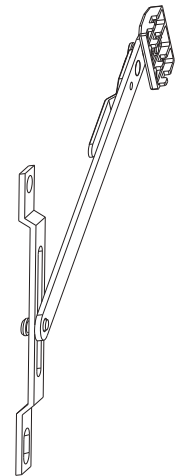
T-90001-00-0-1 Security Plate
