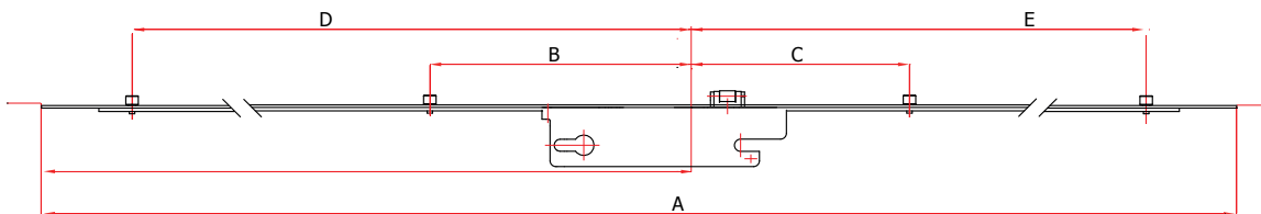
TGP Focus6 Lockable Door Gear, Key Operated, with roller, 35 / 92
